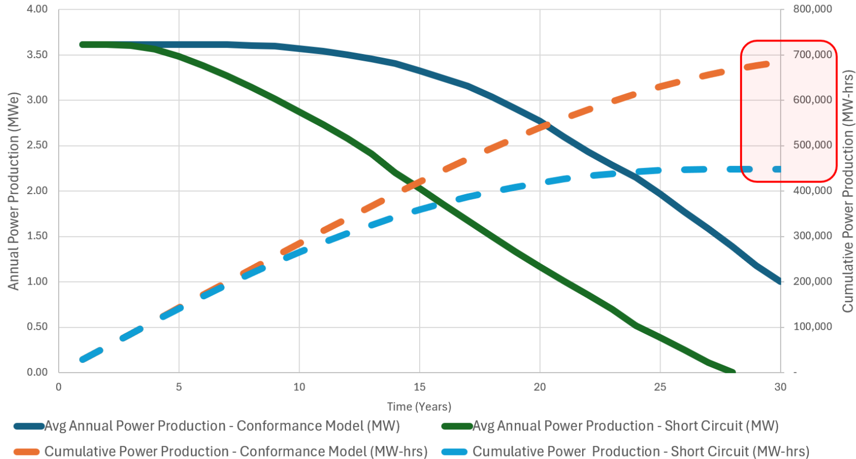
Power Generation Loss Due to Short Circuiting
